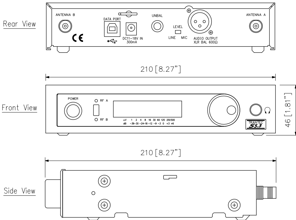
Wireless tuner
