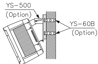
Pole Mounting
